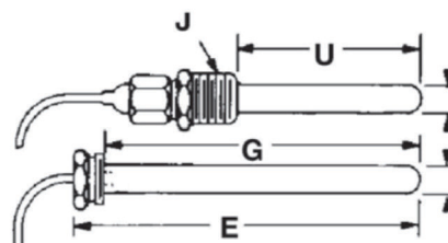
GAS SERVICE BULB & WELL DIMENSIONS INCHES (MM)
