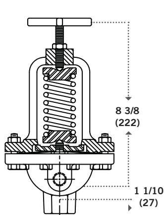
ADJUSTING HANDWHEEL
