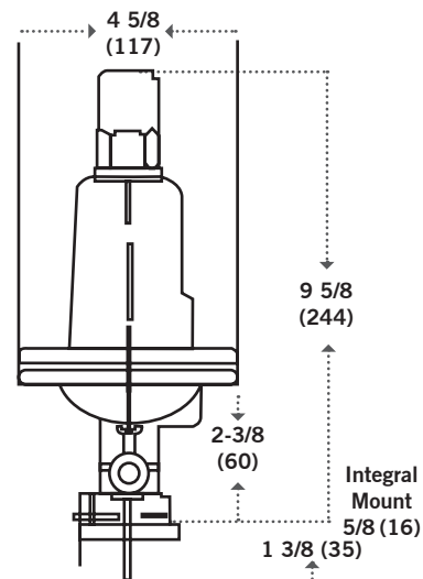
TYPE N PILOT 8 LBS (3.6 KG)
