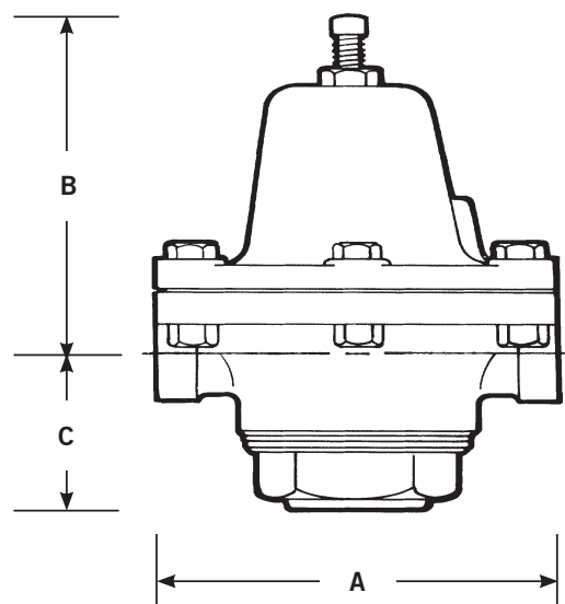
TYPE D50A DIRECT ACTING PRESSURE REDUCING VALVE
