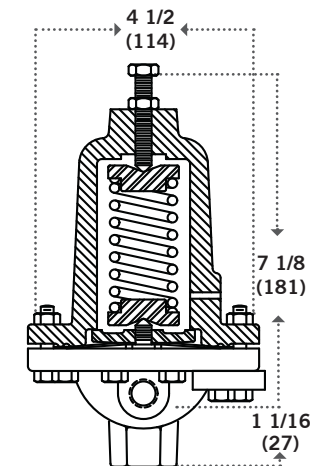
SPRING CHAMBER
