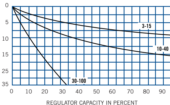
1 1/2" & 2" VALVE DROOP CHART
