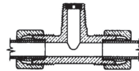
7C ANTI-FREEZE RESTRICTION TEE
