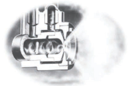
DUAL CONTROL DESUPERHEATER NOZZLE
