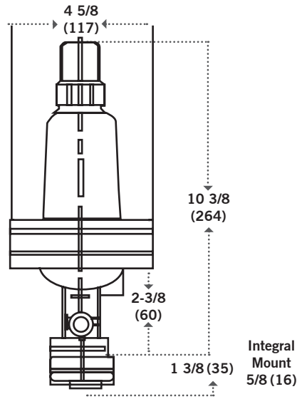
TYPE N33 PILOT 11 LBS (5 KG)
