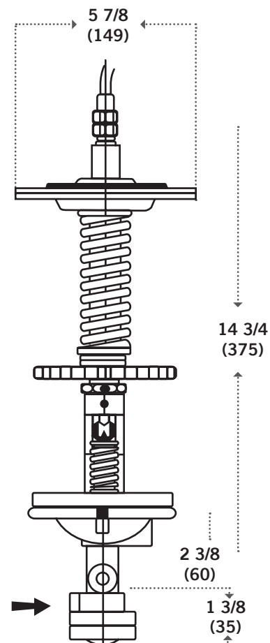
TYPE T124 PILOT 16-LBS. (7.3 KG)
