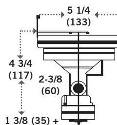
TYPE A43 11 LBS (5 KG)
