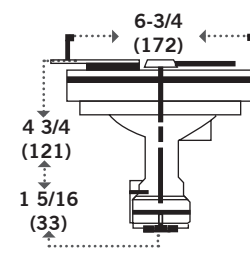
TYPE A54 19 LBS (8.6 KG)
