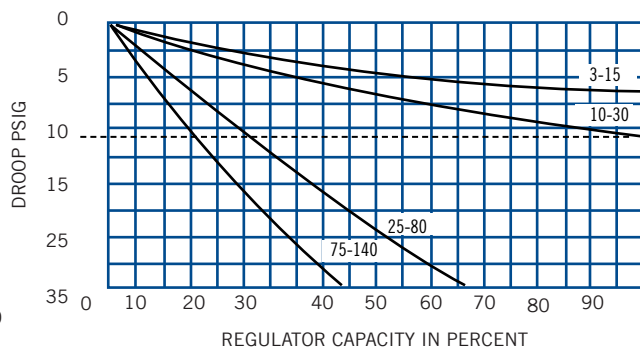
1 1/2" & 2" VALVE DROOP CHART
