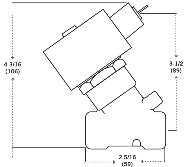
TYPE M33 SOLENOID PILOT 125# 3 LBS. (1.4 KG)
