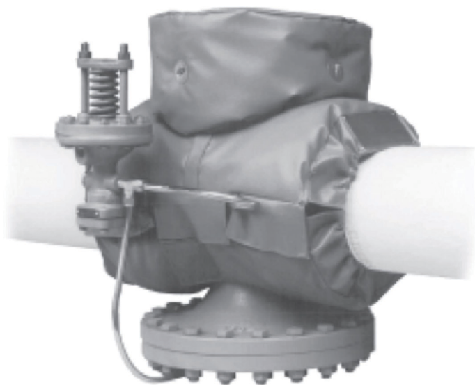
INSULCAP JACKET
