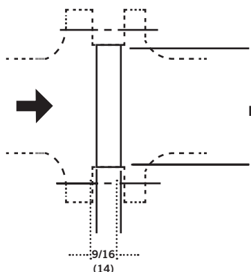
ANSI 250, 300 & 600 FLANGED
