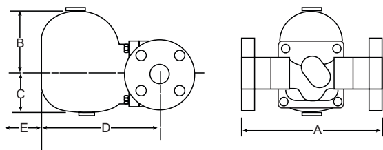
FTE-44F CAST STEEL 1"
