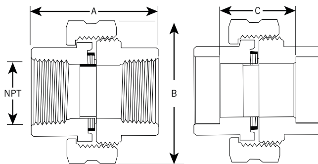
Uniflex Model SUA-T
