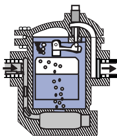
Trap Begins to Open
