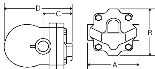
FTE-14-DUCTILE IRON 1/2", 3/4" & 1"
