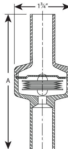
TUBE CONNECTION
