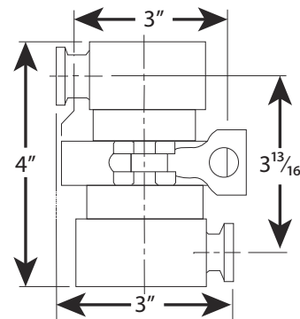
CDH-AI-AO - 3.9 LB.
