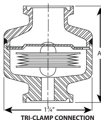
TRI-CLAMP CONNECTION
