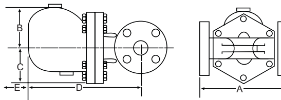
FTE-43 CAST IRON 1 \frac{1}{2} " & 2"
