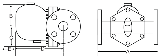
FTE-44F CAST STEEL 1 \frac{1}{2} " & 2"
